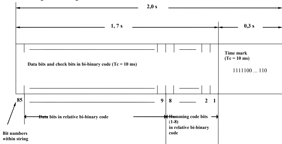
Figure 4.3 String structure
